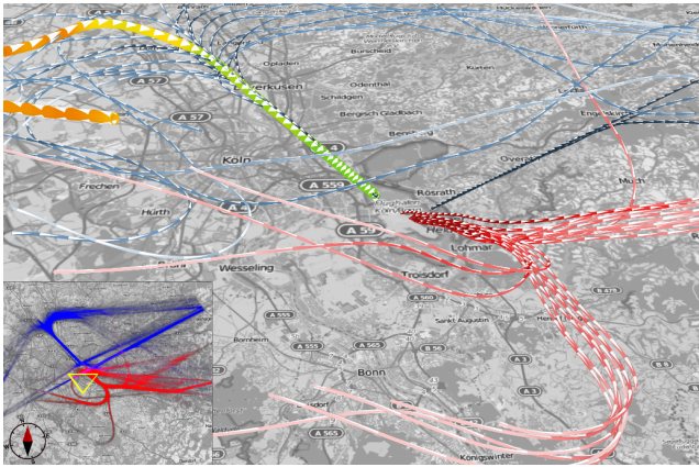
Fig. 10: Example detail+overview visualization, combining density maps with 3D trajectory rendering.
