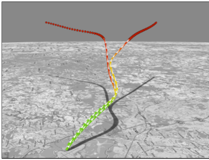
(a) Dynamic mapping of per-node attributes to visual properties. The trajectory is rendered as a tube in the foreground, in the rear, nodes are depicted by spheres. Speed is mapped to color.
