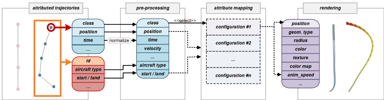
Fig. 4: Schematic mapping overview: attributed nodes and trajectories constitute the input data items for the mapping stage. The primary attribute class selects the actual mapping configuration that is applied. During attribute mapping, input attributes are mapped to visual properties of the visualization technique.
