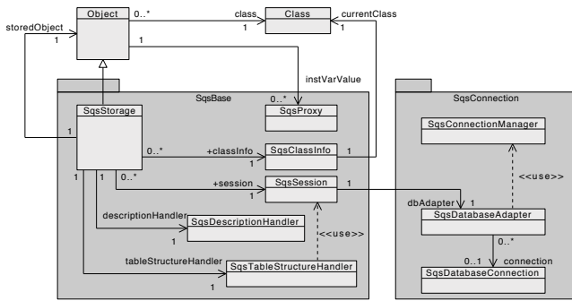
Figure 2: Overview of SqueakSave System Classes
