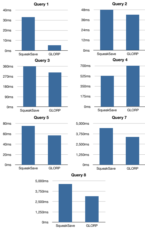
Figure 5: Benchmark Query Times
