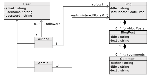
Figure 1: Class Structure of the Example Application.
