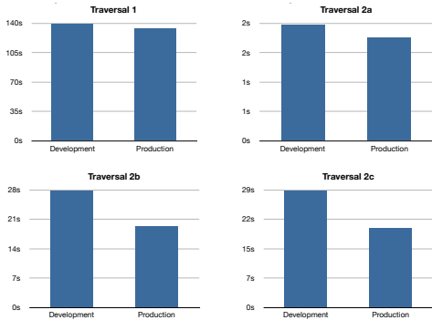
Figure 8: Benchmark Traversal Times for SqueakSave Modes
