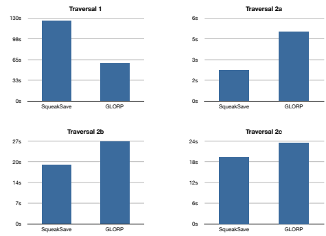
Figure 6: Benchmark Traversal Times
