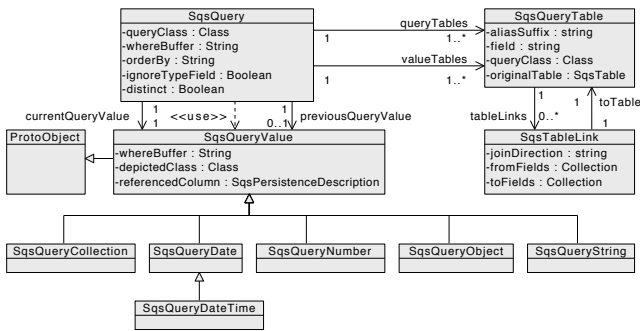
Figure 3: Collection Protocol Emulation Classes
