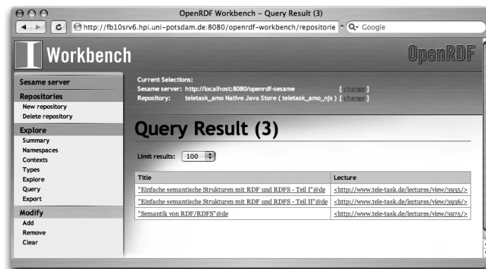
Fig. 5: Sesame server web portal displaying the result of the query in Fig. 4
