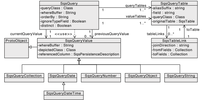
Figure 3. Collection Protocol Emulation Classes
