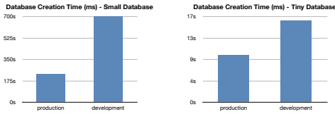
Figure 7. Benchmark Database Creation Times for SqueakSave Modes
