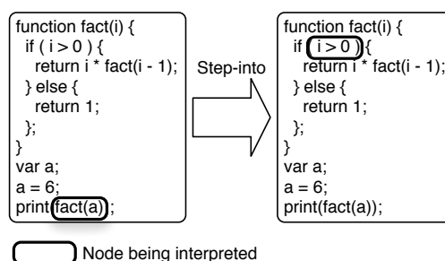
Figure 4: A step-into operation goes into recursion.
