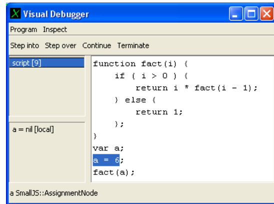
Figure 2: A graphical user interface of a debugger.
